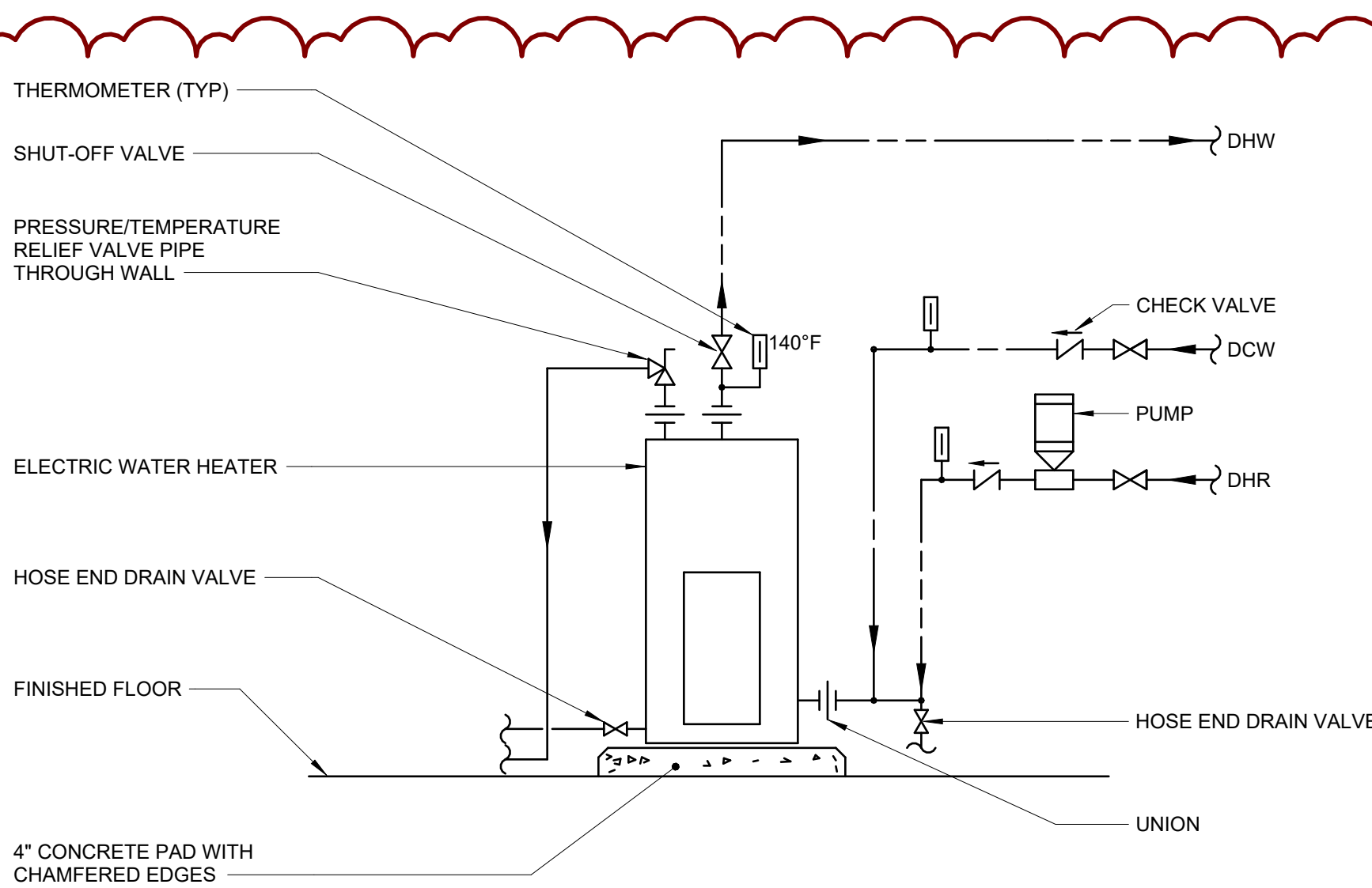
2 DETAIL - ELECTRIC WATER HEATER (WITH RECIRC PUMP) SCALE: N.T.S.
